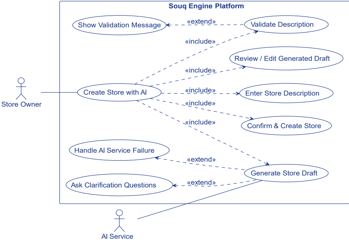
Use Case Diagram: AI Store Creation
